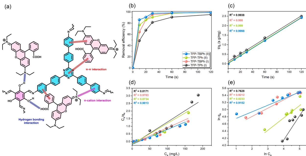
Fig. 9. (a) Possible RhB adsorption mechanisms of TFP COFs; (b) removal efficiency of aqueous RhB at different times after the addition, (c) pseudo-second-order kinetic fitting, (d) Langmuir fitting, and (e) Freundlich fitting of TFP COFs.
