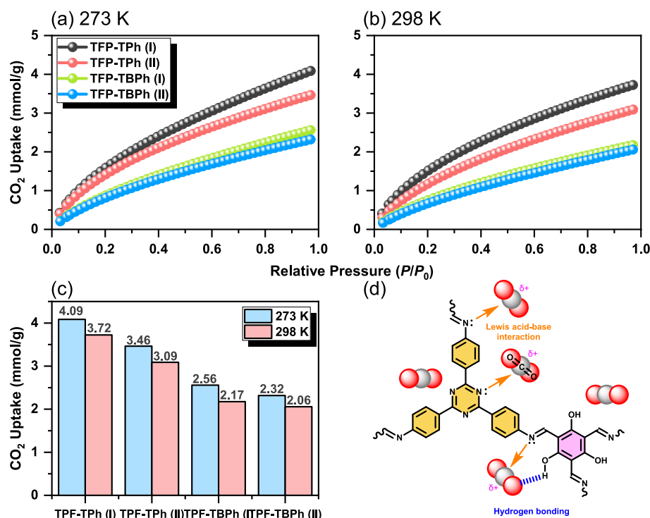
Fig. 7. CO 2 adsorption profiles of TFP COFs at (a) 273 K, (b) 298 K, and (c) summarize their corresponding CO 2 uptake values. (d) Proposed mechanism of CO 2 adsorption in TFP-Based COFs.
