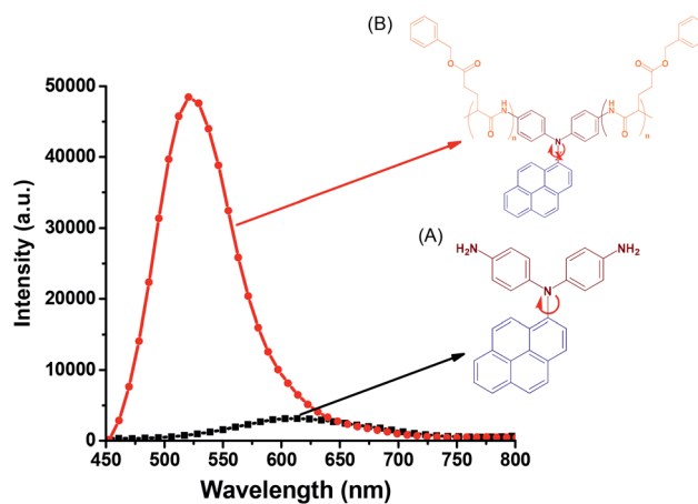
Fig. 7 Solution PL emission spectra of (A) pyrene-DPA-2NH 2 and (B) pyrene-DPA-PBLG(6) in THF (concentration: 10 −3 M; excitation wavelength: 343 nm).
