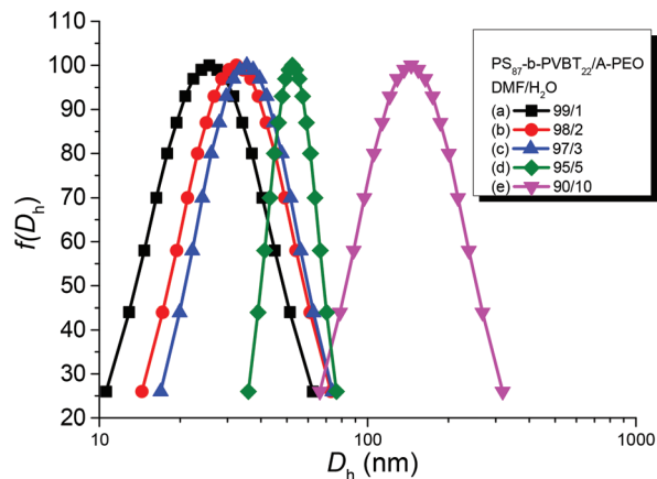
Fig. 3 DLS data for the PS 87 - b -PVBT 22 /A-PEO supramolecular complexes formed in DMF/H 2 O solutions at various water contents of (a) 1, (b) 2, (c) 3, (d) 5, and (e) 10 wt%.
