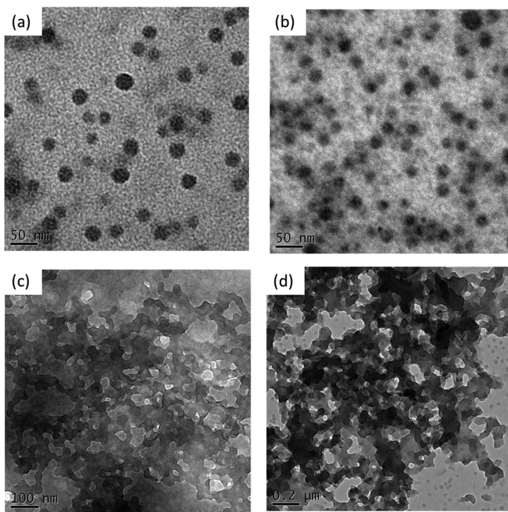
Fig. 1 TEM images of the PS 87 - b -PVBT 22 /A-PEO supramolecular complexes formed in DMF/H 2 O solutions containing various water contents of (a) 1, (b) 2, (c) 5, and (d) 10 wt%.
