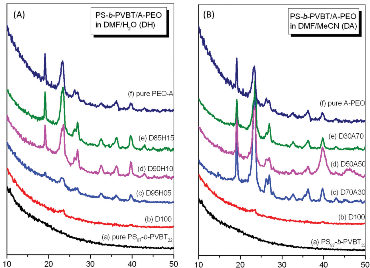
Fig. 13 WAXD patterns of PS_{87}\text{-}b\text{-}PVBT_{22}/A\text{-}PEO supramolecular complexes formed at various contents of the selective solvent: (A) DMF/ H_2O and (B) DMF/MeCN solutions.
