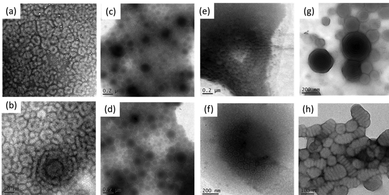
Fig. 10 TEM images of PS 87 - b -PVBT 22 /A-PEO supramolecular complexes formed in DMF/MeCN solution at a MeCN content of 70 wt% at T/A ratios of (a and b) 1 : 0.3, (c and d) 1 : 0.5, (e and f) 1 : 0.7, and (g and h) 1 : 1.
