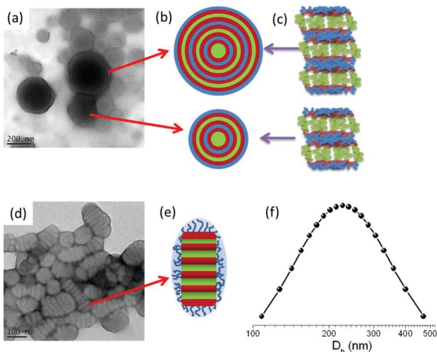
Fig. 9 (a and d) TEM images of the PS 87 - b -PVBT 22 /A-PEO supramolecular complex in DMF/MeCN solution at a MeCN content of 70 wt%. (b and c) Schematic representation of the possible onion sphere structure observed in the TEM image in (a). (e) Schematic representation of the possible wood-louse structure observed in the TEM image in (d). (f) Size-distribution of the micelles by using DLS, corresponding to the TEM images in (a) and (d).
