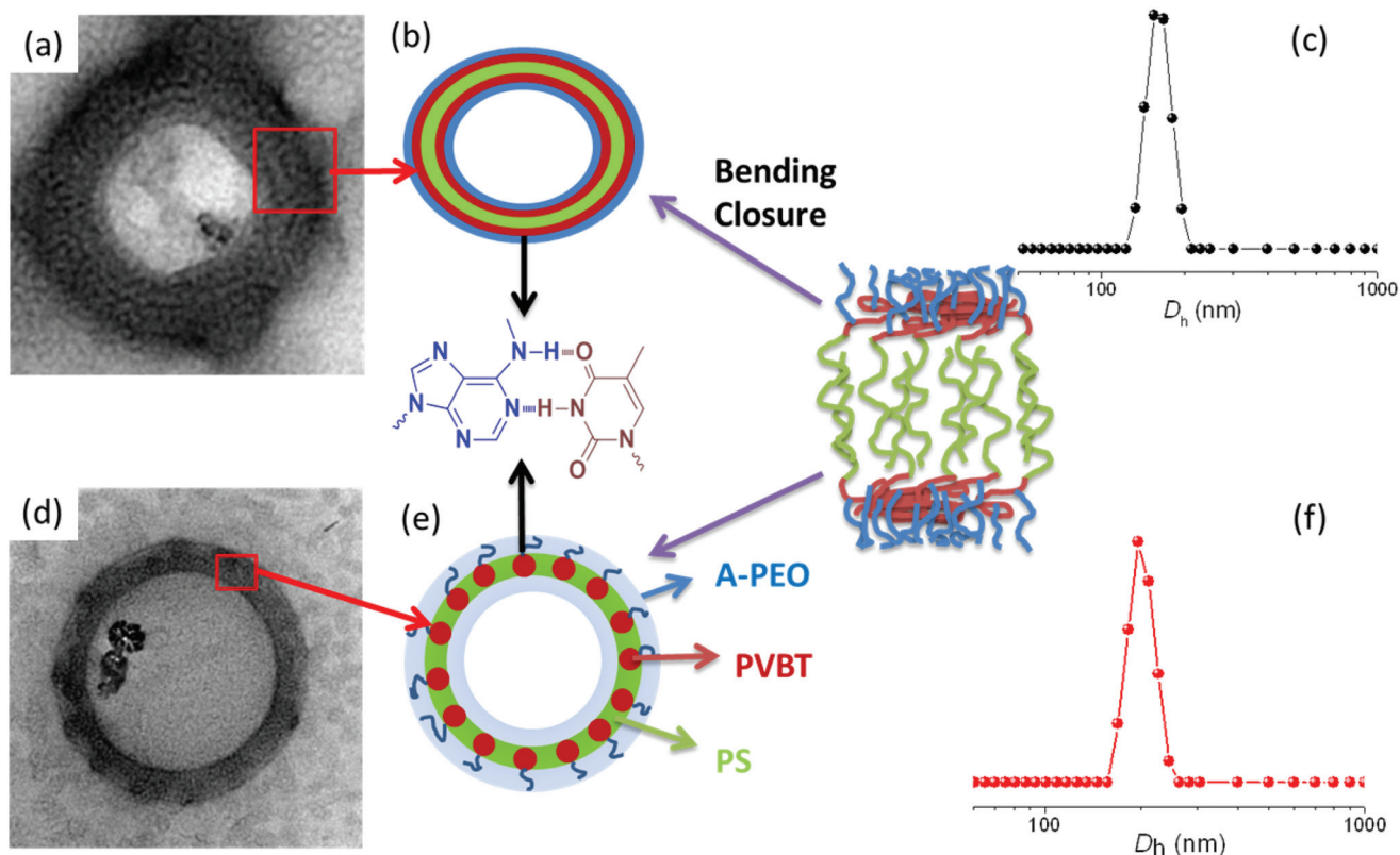
Fig. 5 (a) Expanded TEM images of the PS_{67} - b - PVBT_{16} /A-PEO supramolecular complex formed in DMF/ H_2O solution at 10 wt% water content. (b) Schematic representation of the possible layer-vesicle structure observed in the TEM image in (a). (c) Size-distribution of the micelles by using DLS. (d) TEM image of the PS_{67} - b - PVBT_{16} /A-PEO supramolecular complex formed in DMF/ H_2O solution at 25 wt% water content. (e) Schematic representation of the possible in-plane layer vesicle structure observed in (d). (f) Size-distribution of the micelles by using DLS, corresponding to the TEM image in (d).
