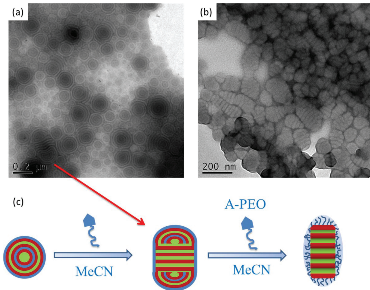
Fig. 12 TEM images of PS 87 - b -PVBT 22 /A-PEO supramolecular complexes formed at T/A ratios of (a) 1:0.5 and (b) 1:1. (c) Possible morphologies, from onion structures to woodlouse structures, formed in the DMF/MeCN solution at a MeCN content of 70 wt%.
