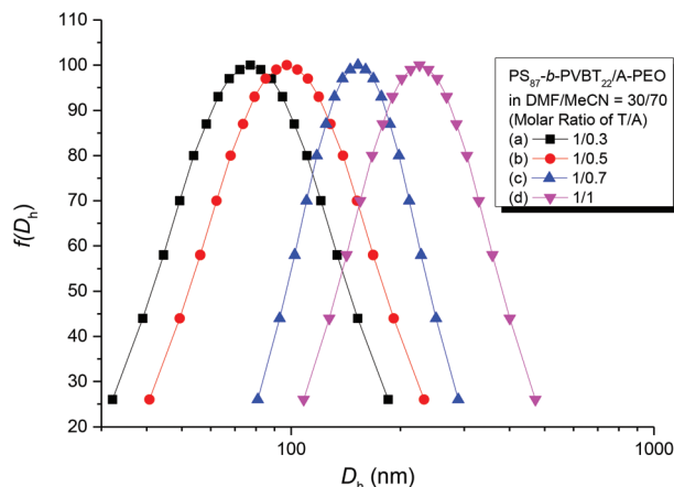
Fig. 11 DLS data of PS 87 - b -PVBT 22 /A-PEO supramolecular complexes formed in DMF/MeCN solution at a MeCN content of 70 wt% at T/A ratios of (a) 1 : 0.3, (b) 1 : 0.5, (c) 1 : 0.7, and (d) 1 : 1.
