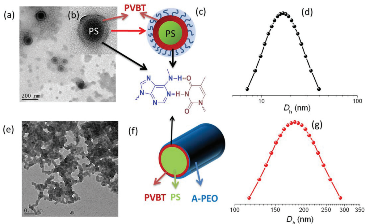
Fig. 8 (a and b) Expanded TEM images of the PS 87 - b -PVBT 22 /A-PEO supramolecular complex formed in DMF/MeCN solution at a MeCN content of 10 wt%. (c) Schematic representation of the possible core-shell-corona sphere morphology observed in the TEM image in (b). (d) Size-distribution of the micelle corresponding to the TEM image in (a) by using DLS. (e) TEM image of the PS 87 - b -PVBT 22 /A-PEO supramolecular complex formed in DMF/MeCN solution at a MeCN content of 30 wt%. (f) Schematic representation of the possible core-shell-corona cylinder morphology observed in the TEM image in (e). (g) Size-distribution of the micelles by using DLS, corresponding to the TEM image in (e).
