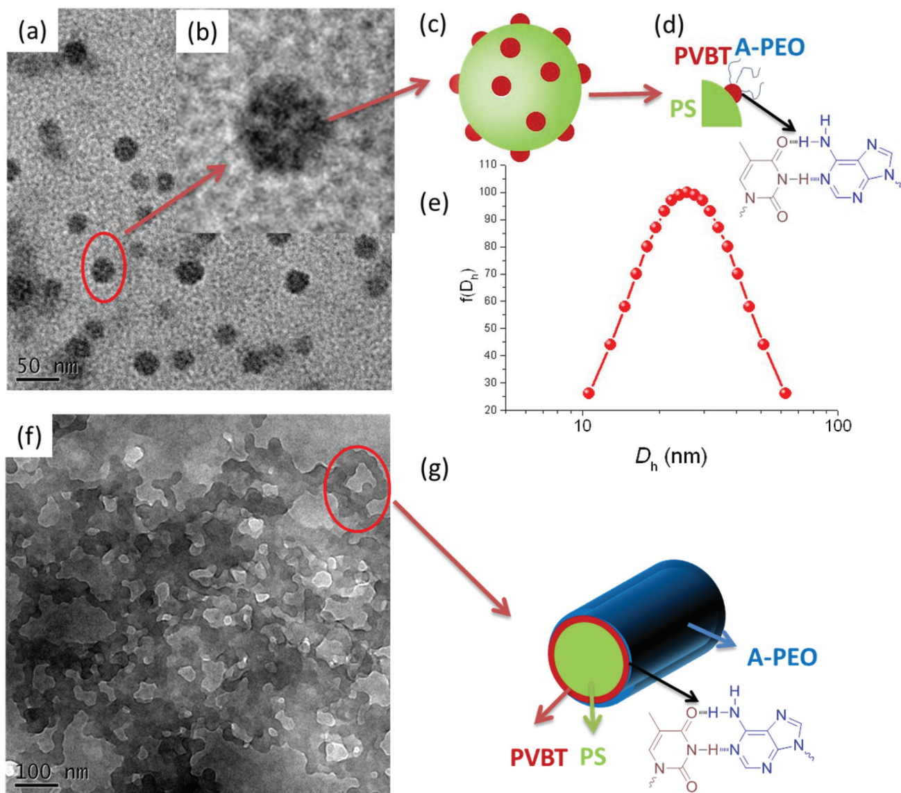
Fig. 2 (a) TEM image of PS 87 - b -PVBT 22 /A-PEO supramolecular complex formed in DMF/H 2 O solution at 1 wt% water content. Inset (b): Magnified image of (a). (c–d) Schematic representation of the raspberry-like spheres in (a). (e) Size-distribution of the micelles by DLS. (f) TEM image of the PS 87 - b -PVBT 22 /A-PEO supramolecular complex formed in DMF/H 2 O solution at 5 wt% water content. (g) Schematic representation of a possible structure for the core–shell–corona cylinder morphology observed in the TEM image in (f).
