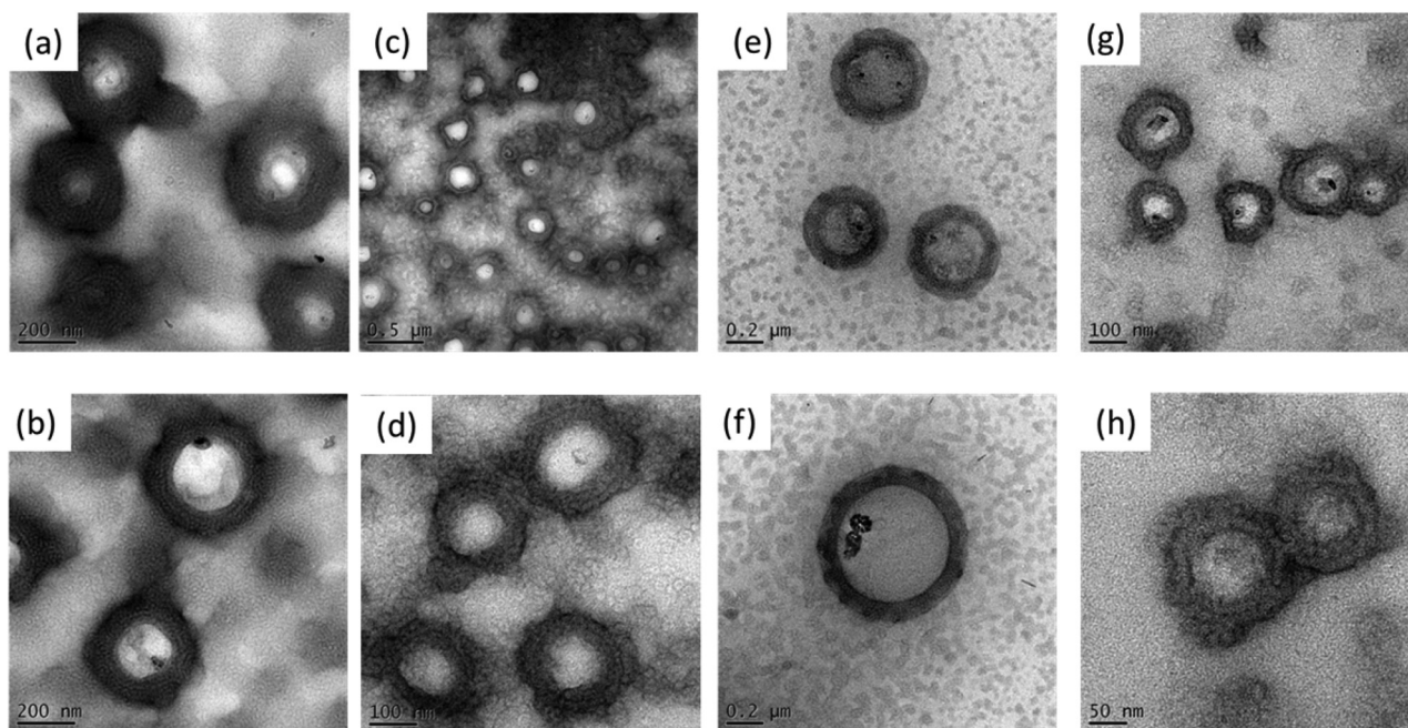
Fig. 4 TEM images of the PS_{67} - b - PVBT_{16} /A-PEO supramolecular complexes formed in DMF/ H_2O solutions at various water contents of (a and b) 10, (c and d) 15, (e and f) 25, and (g and h) 35 wt%.
