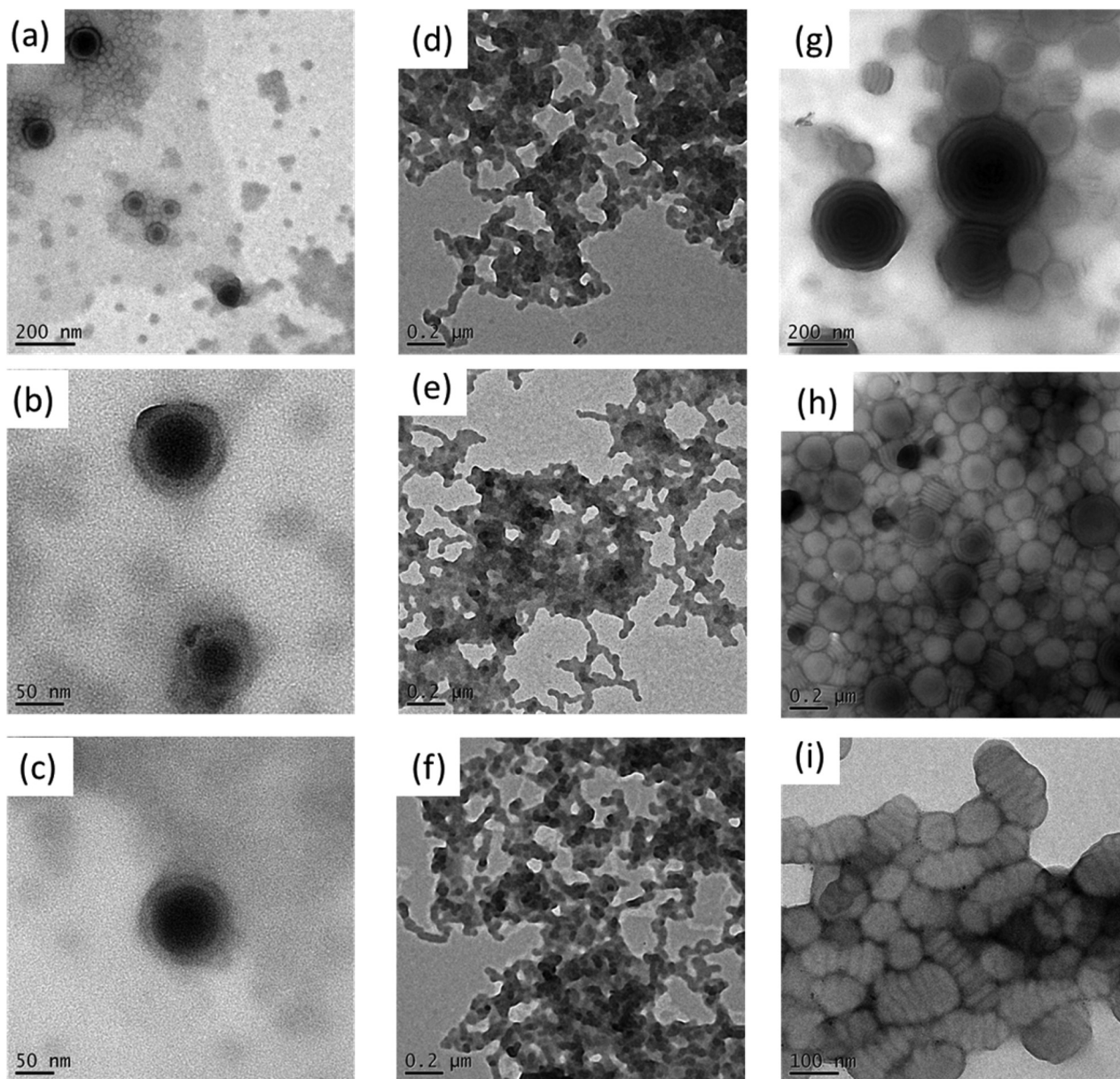
Fig. 7 TEM images of the PS 87 - b -PVBT 22 /A-PEO supramolecular complexes formed in DMF/MeCN solution at various MeCN contents of (a–c) 10, (d–f) 30, and (g–i) 70 wt%.
