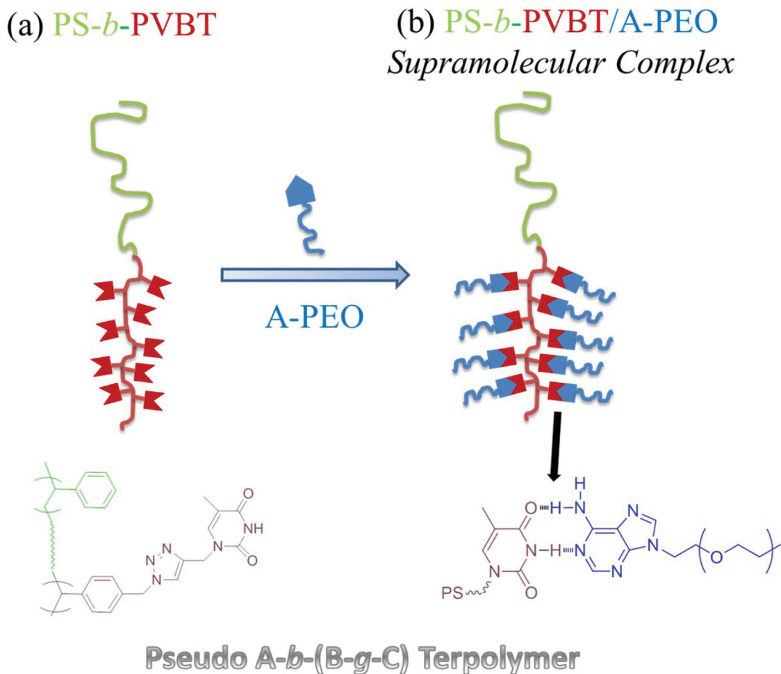
Scheme 1 Cartoon representations of (a) PS- b -PVBT and (b) the supramolecular complex PS- b -PVBT/A-PEO, with the chemical structure of the interaction between the T and A units.
