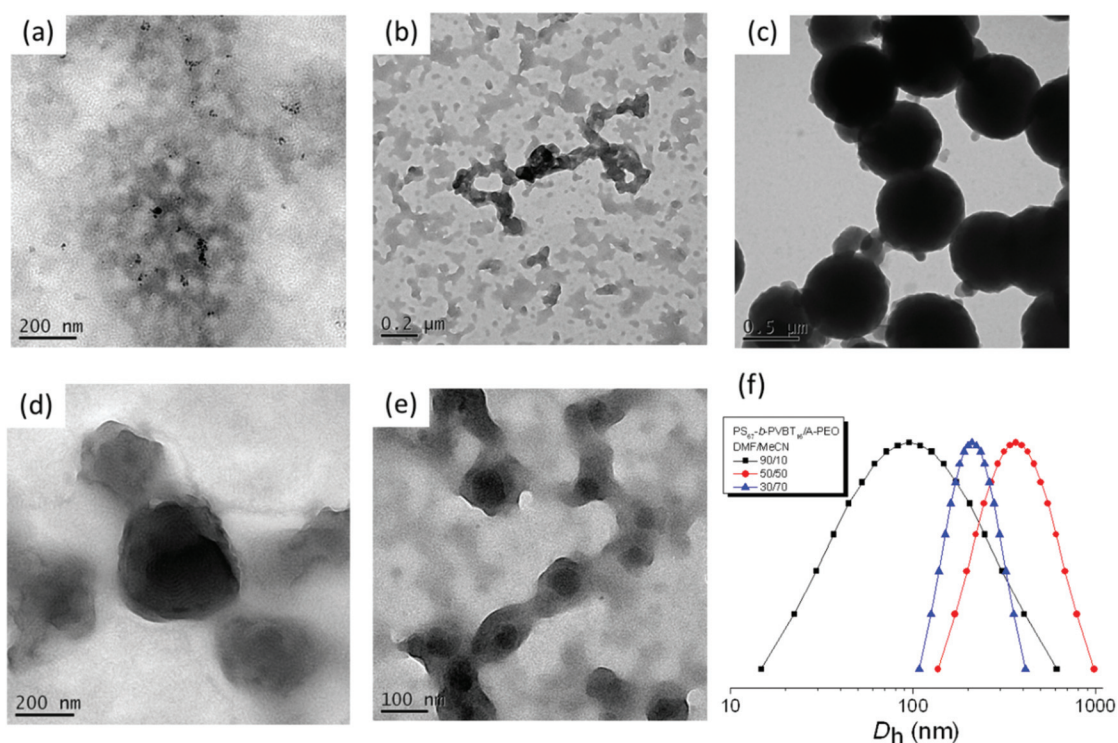
Fig. 6 (a–e) TEM images of the \text{PS}_{67}\text{-}b\text{-PVBT}_{16}/\text{A-PEO} supramolecular complexes formed in DMF/MeCN solution at various MeCN contents of (a) 10, (b) 30, (c) 40, (d) 50, and (e) 70 wt%. (f) Corresponding size-distributions of the micelles by using DLS.
