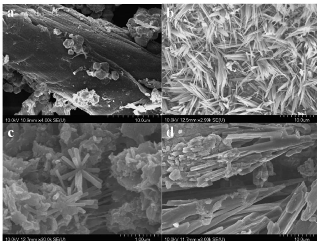
Fig. 8 SEM images displaying the morphologies of the products fabricated using the MPT76 system: M = (a) Cu, (b) Fe, (c) Zn, and (d) Ti.
