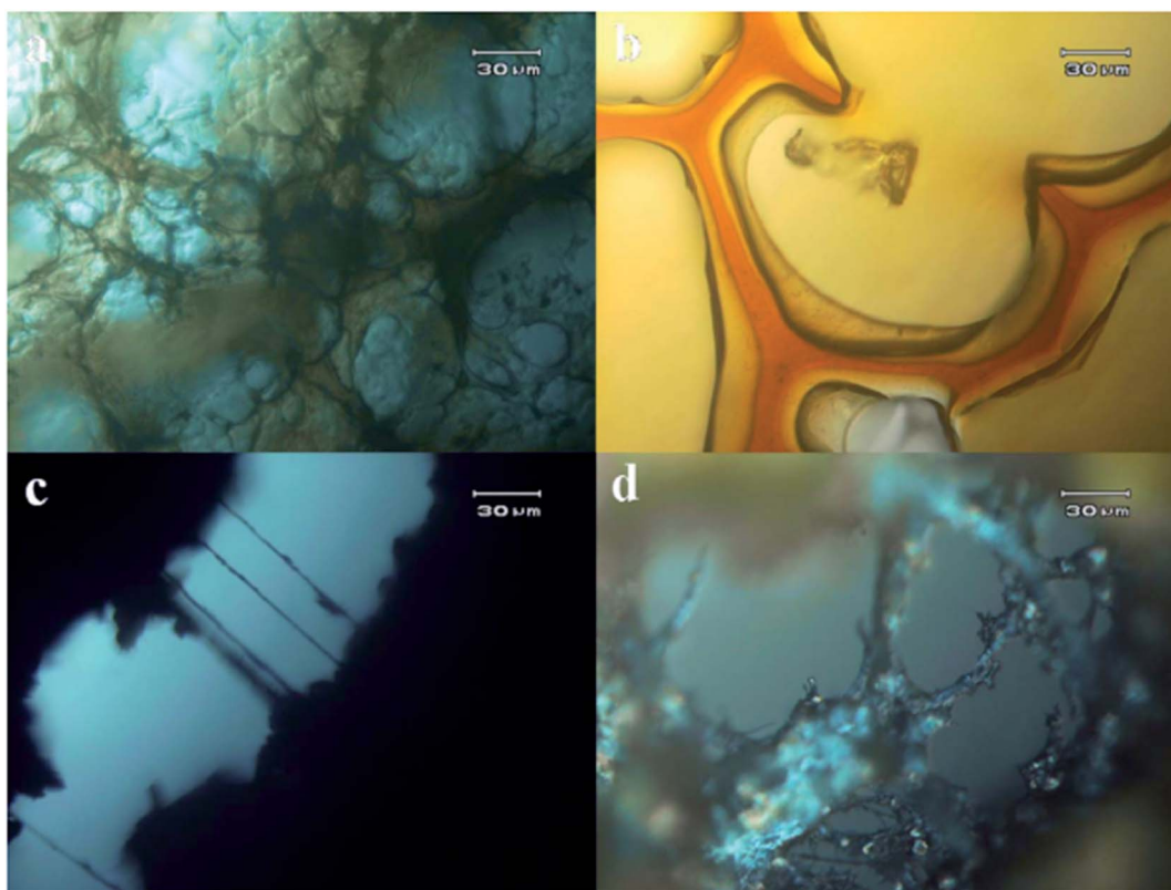
Fig. 3 OM images displaying the morphologies of the products fabricated using the MPT114 system: M = (a) Cu, (b) Fe, (c) Zn, and (d) Ti.
