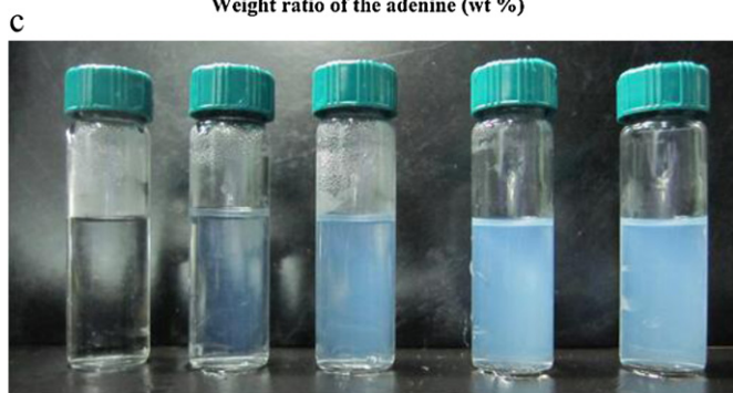
Fig. 2. (a) Turbidimetry analysis of PNIPAAm and the PNIPAAm–adenine complexes P80A20, P50A50, and P20A80 in aqueous solution. The data were obtained upon heating from 25 °C up to a temperature at which a transmittance plateau was clearly defined. A similar profile was obtained upon cooling, with no significant hysteresis. (b) LCSTs of these complexes, recorded as a function of the adenine content. (c) Photographs of aqueous solutions at 45 °C of (from left to right) pure adenine, P20A80, P50A50, P80A20, and pure PNIPAAm.
