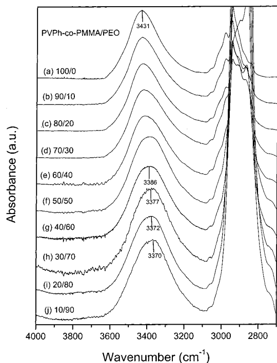
Figure 12. FTIR spectra recorded at 150 °C at 2700 \text{cm}^{-1} –4000 \text{cm}^{-1} region for various PVPh- co -PMMA/PEO blends: (a) 100/0; (b) 90/10; (c) 80/20; (d) 70/30; (e) 60/40; (f) 50/50; (g) 40/60; (h) 30/70; (i) 20/80; (j) 10/90.
