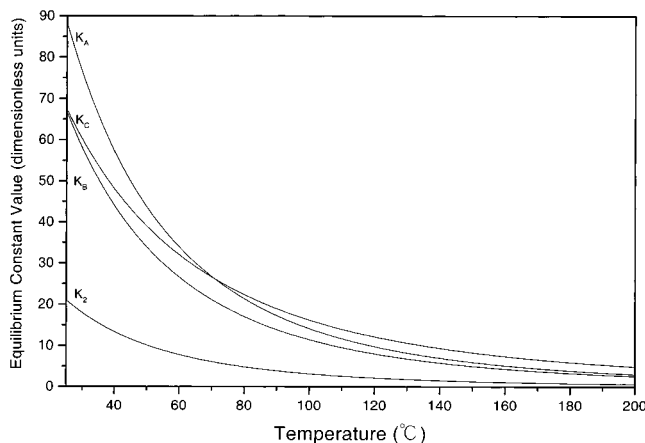
Figure 13. Equilibrium constant values as a function of temperature from 25 to 200 °C.
